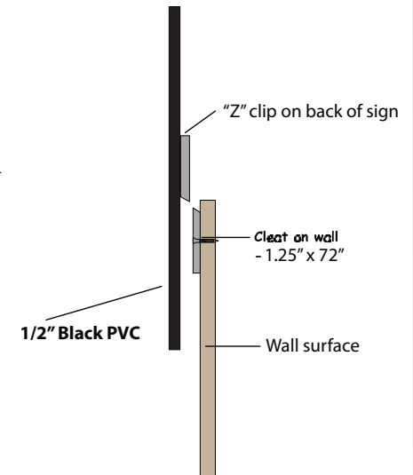
Side View Cleat Hardware
